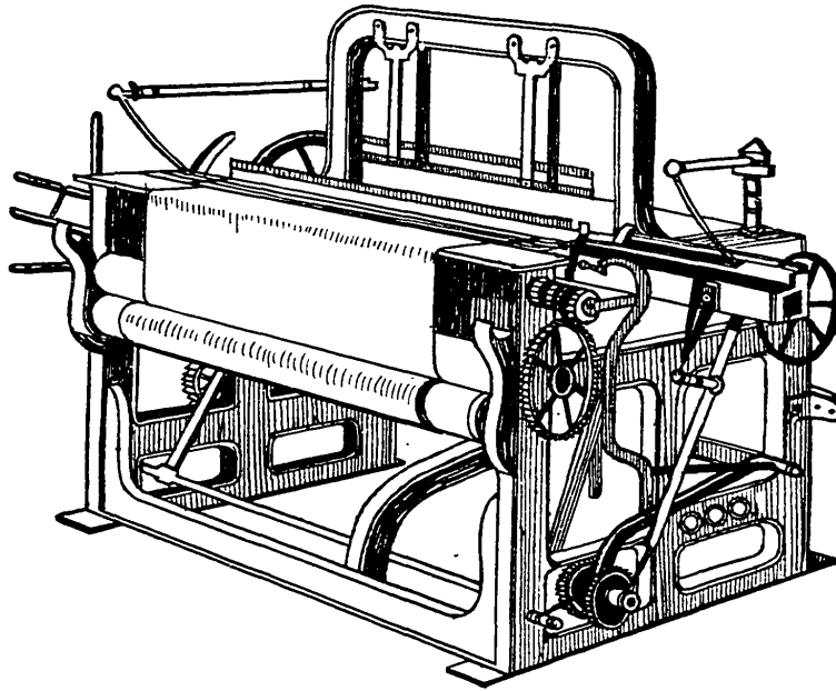
ENGLISH POWER LOOM FOR WEAVING COTTON, 1847
